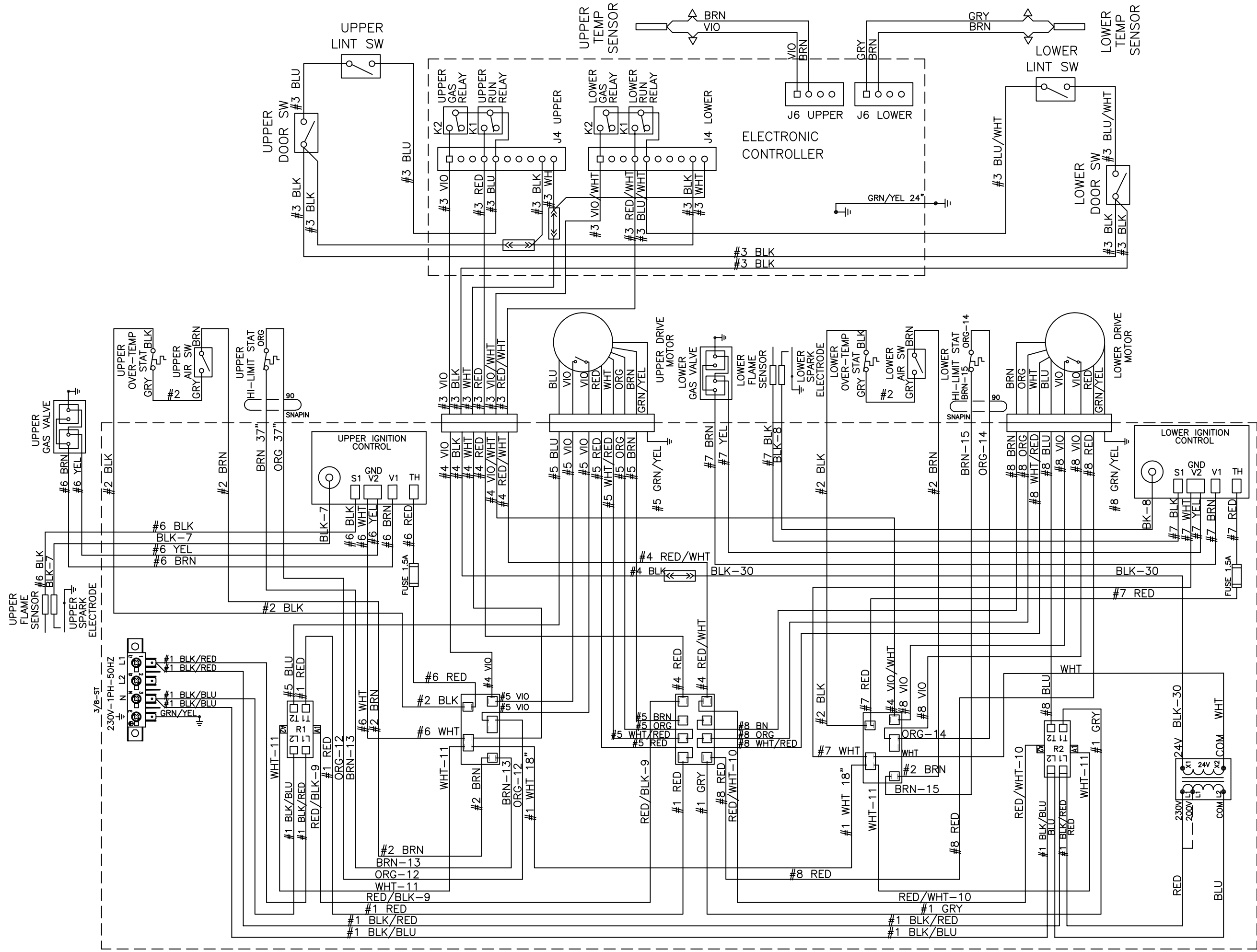
9506-839-001B WIRING DIAGRAM DN20X2N_-39AB_X-
