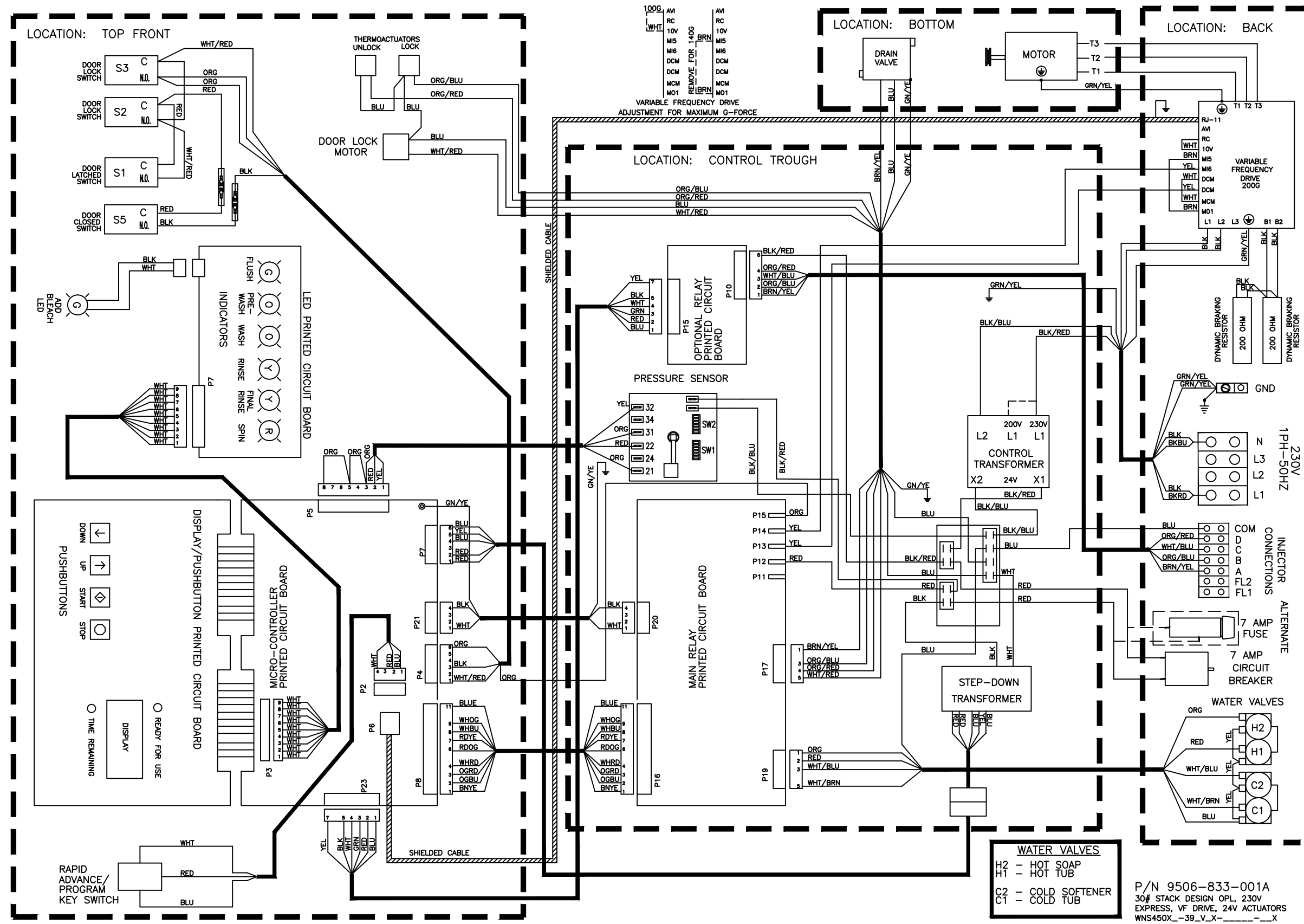
WIRING DIAGRAM 230V, 1PH, 50HZ
