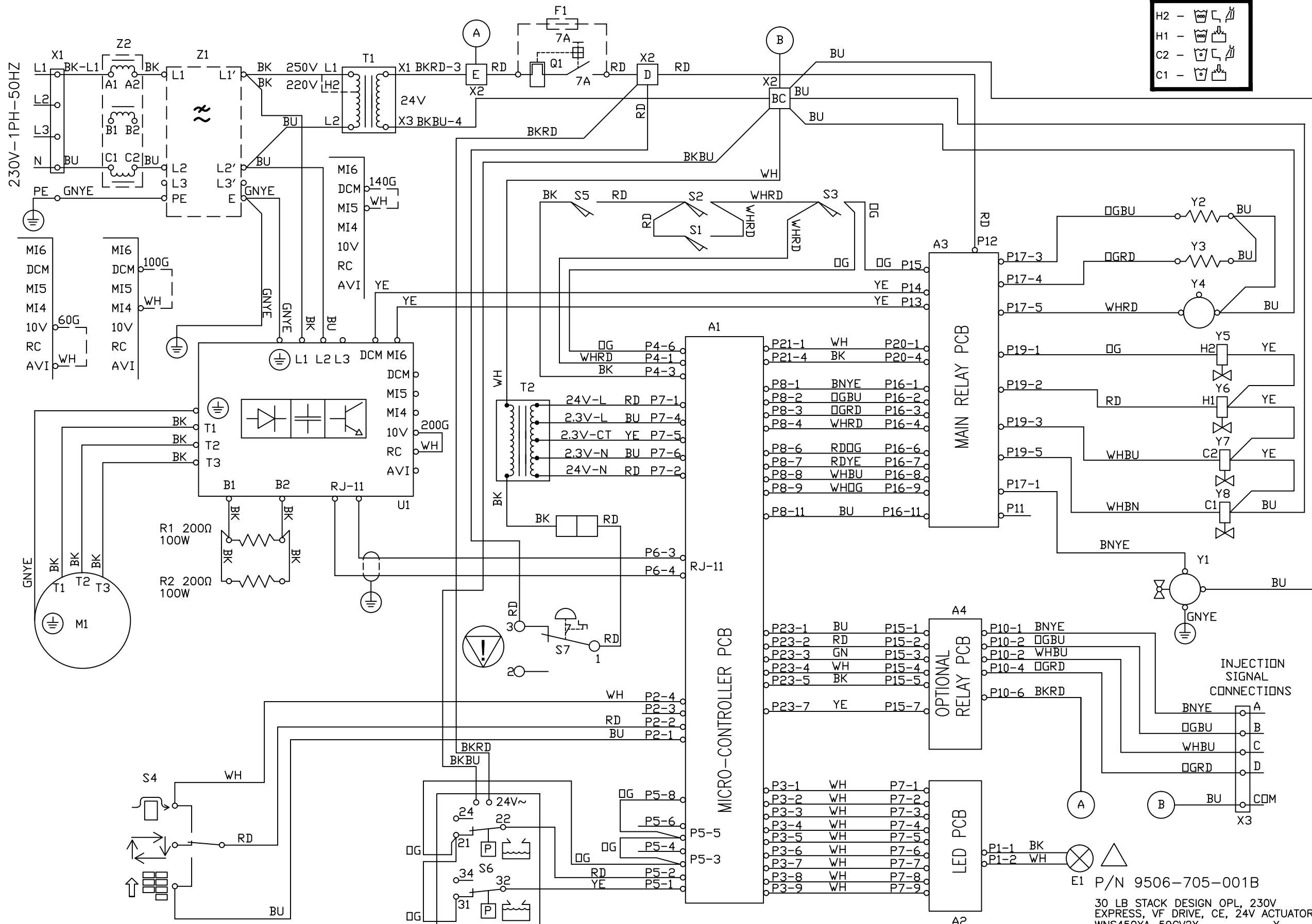
SCHMATIC 230V, 1PH, 50HZ 30 LB STACK DESIGN OPL, 230V EXPRESS, VF DRIVE, CE, 24V ACTUATORS WNS450XA-59CV2X-_____X
