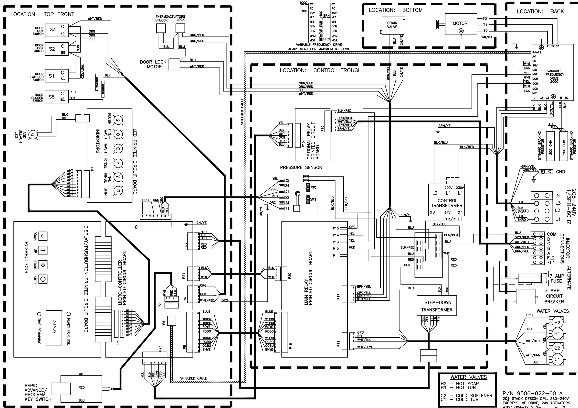
WIRING DIAGRAM 208-240V, 1-3PH, 60HZ
