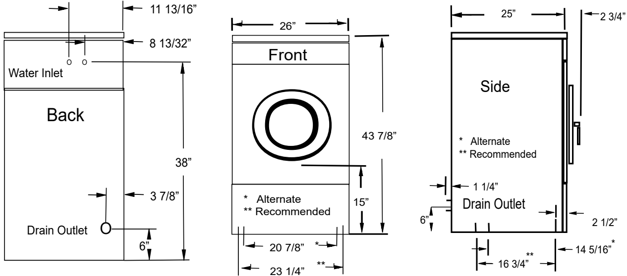
T-300 Mounting Dimensions
