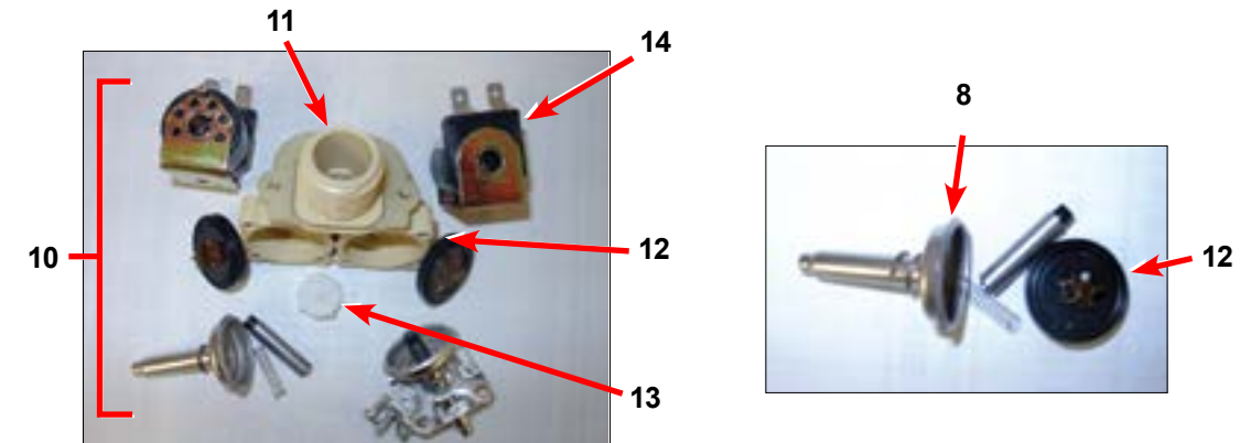
Mueller Valve
