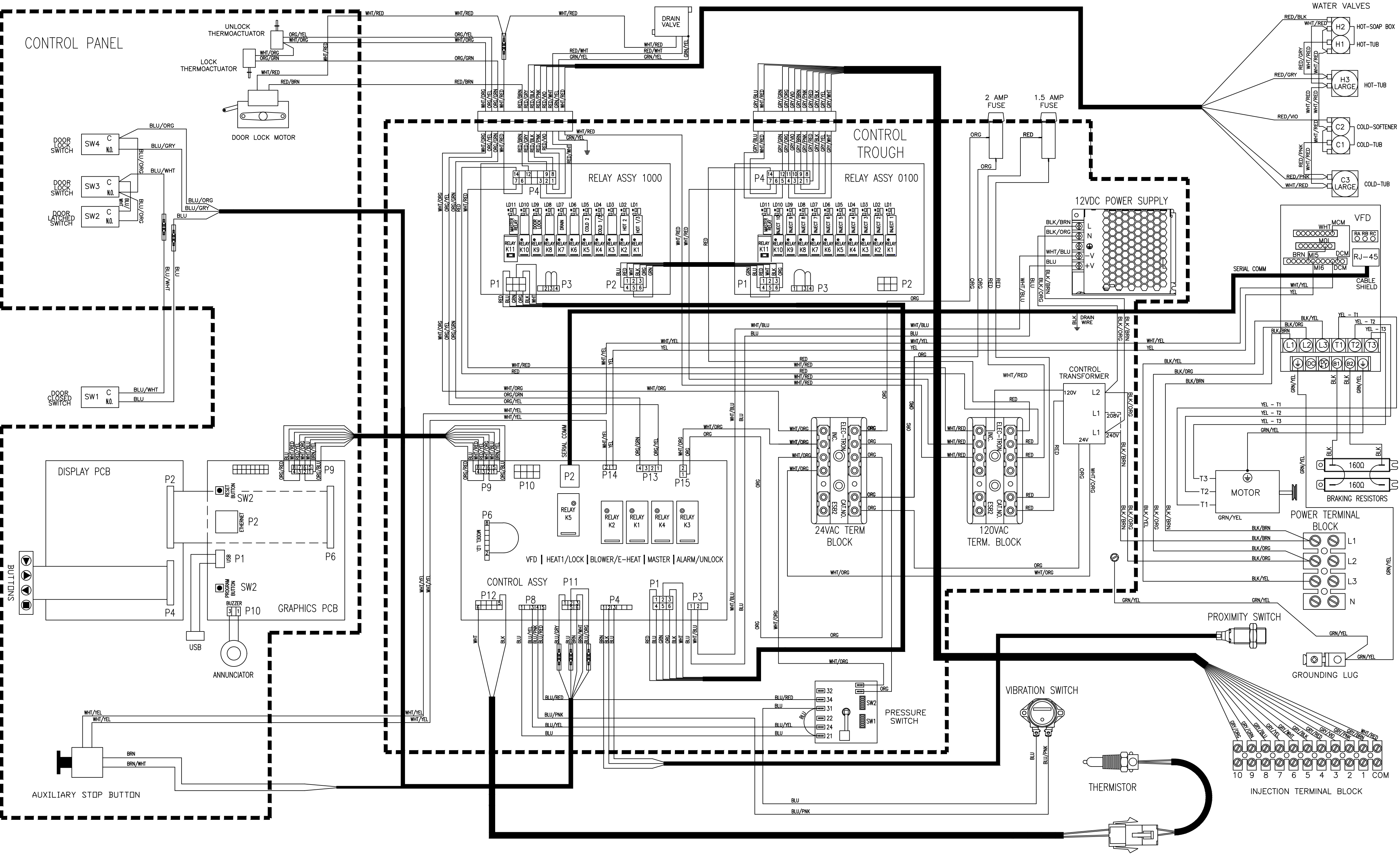
WIRING DIAGRAM 208 - 240V, 1/3PH, 60HZ
