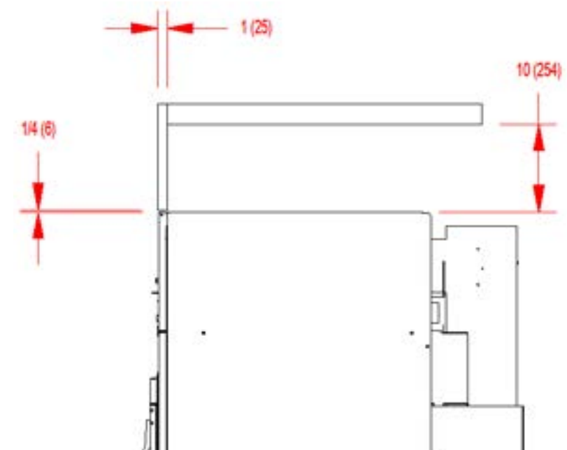
VERTICAL CLEARANCE DIMENSIONS - ALL (30/50/80)
