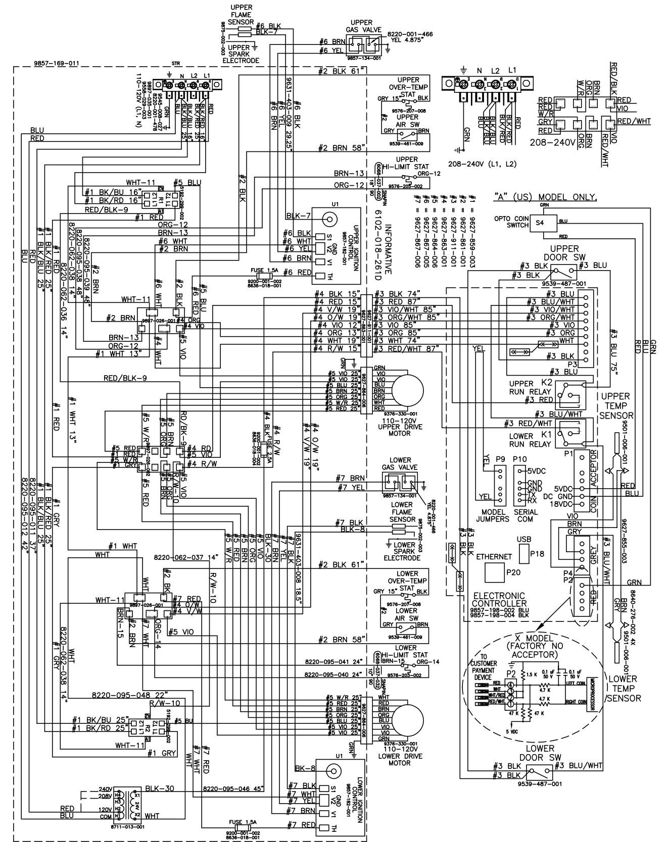
9506-595-001B WIRING DIAGRAM DC30X2NC-15EC2X-
