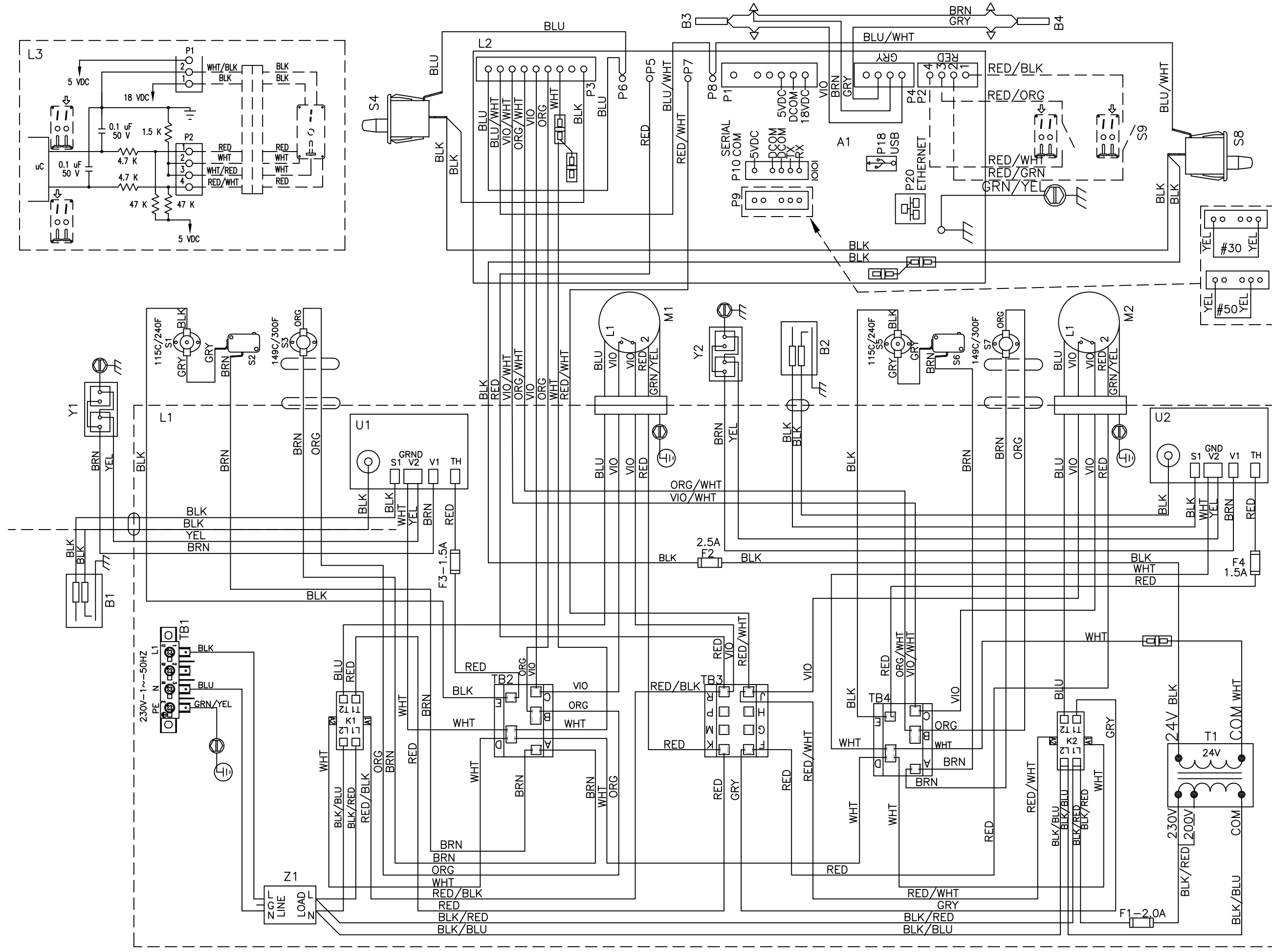
9506-965-001R WIRING DIAGRAM DC(30/50)X2N_59CC_X-
