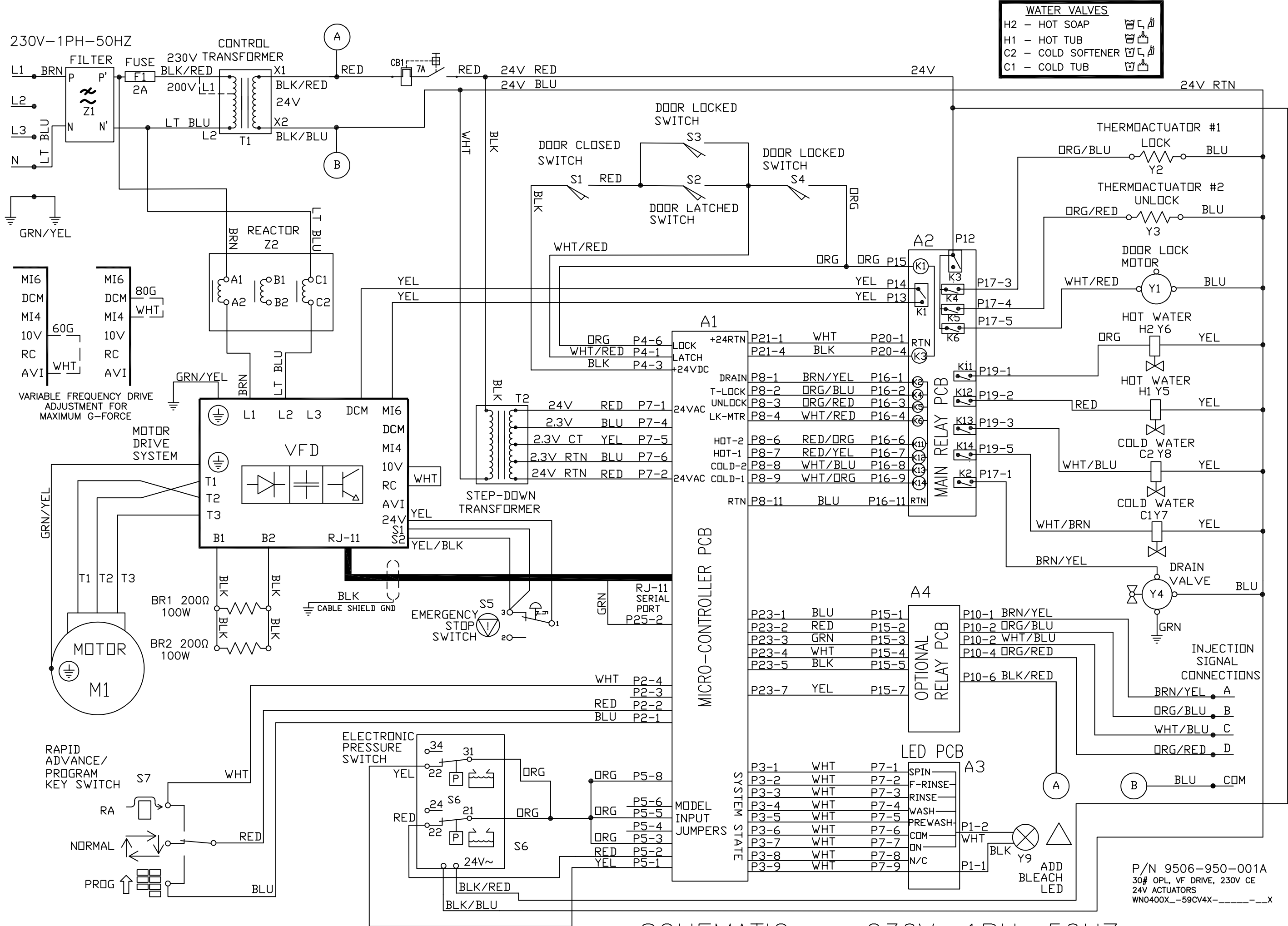
SCHMATIC 230V, 1PH, 50HZ
