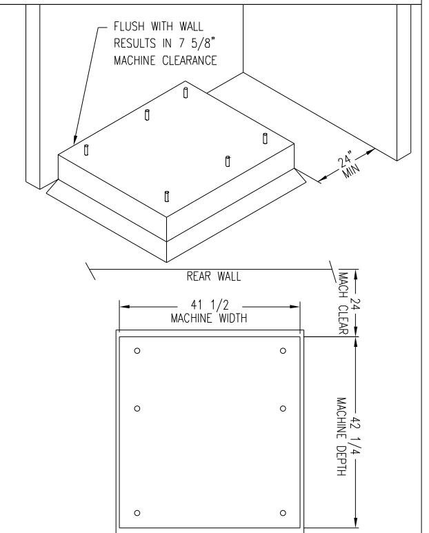
FLOOR OUTLINE
