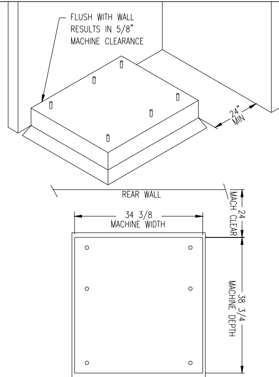
FLOOR OUTLINE
