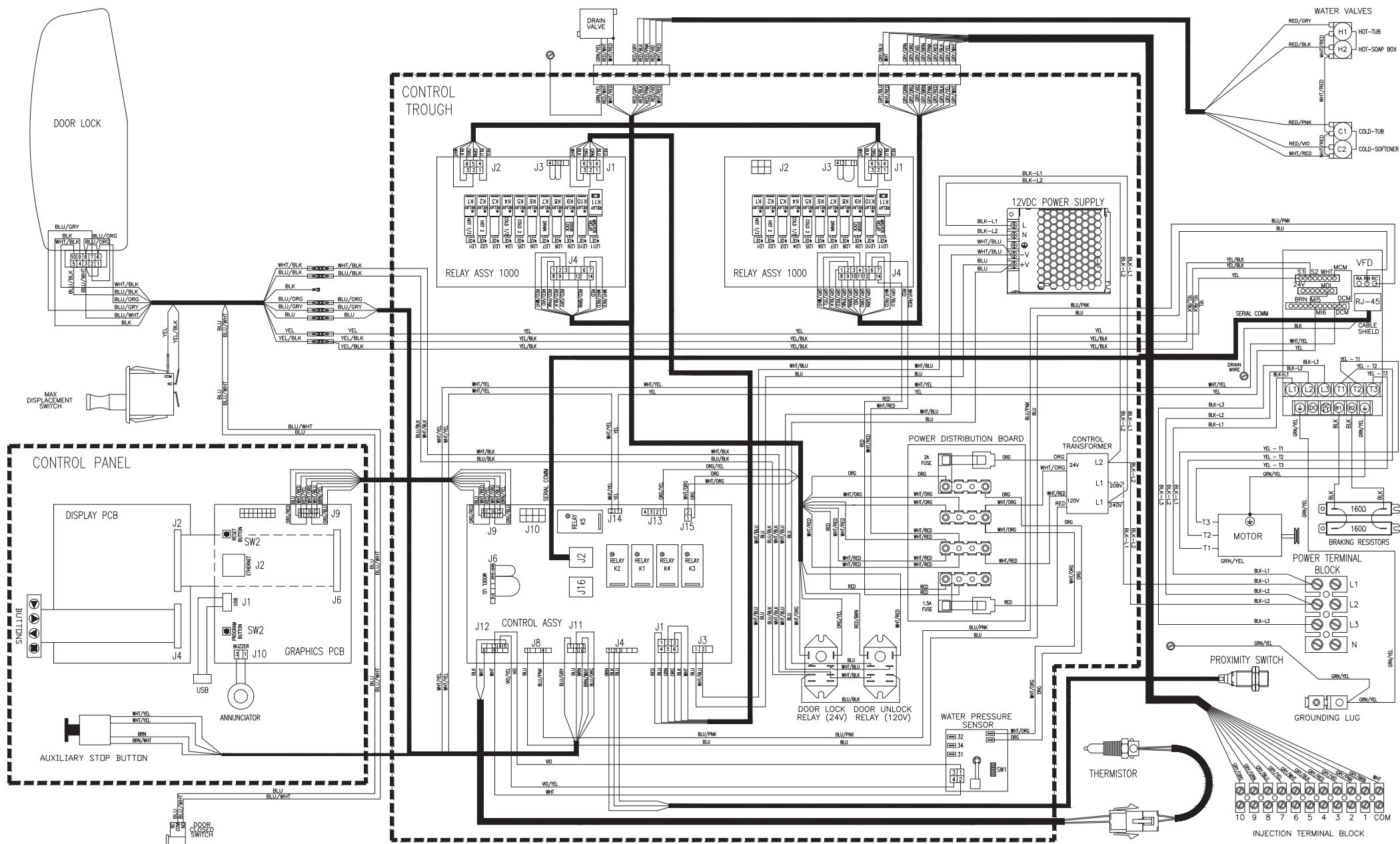
WIRING DIAGRAM 208 - 240V, 1/3PH, 60HZ
