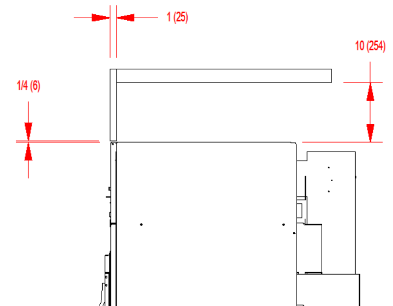
Vertical Clearance Dimension
