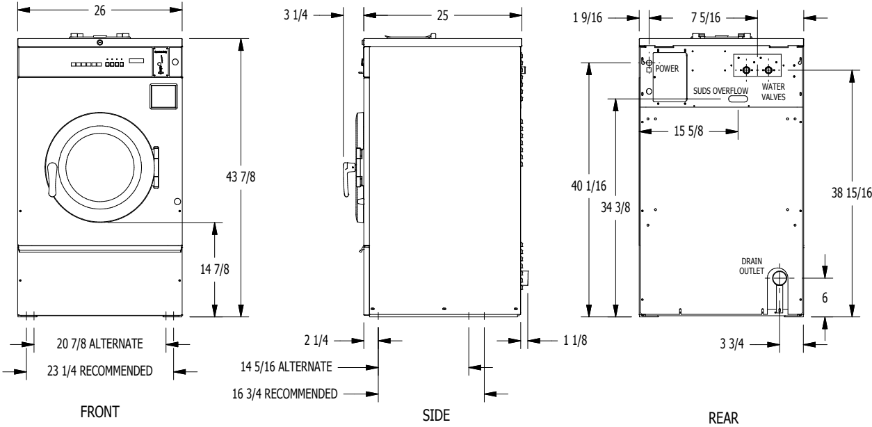
T-300 Mounting Dimensions
