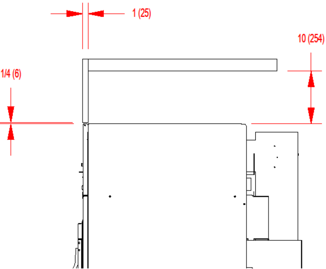
VERTICAL CLEARANCE DIMENSIONS - ALL DCBD(30/50/80)
