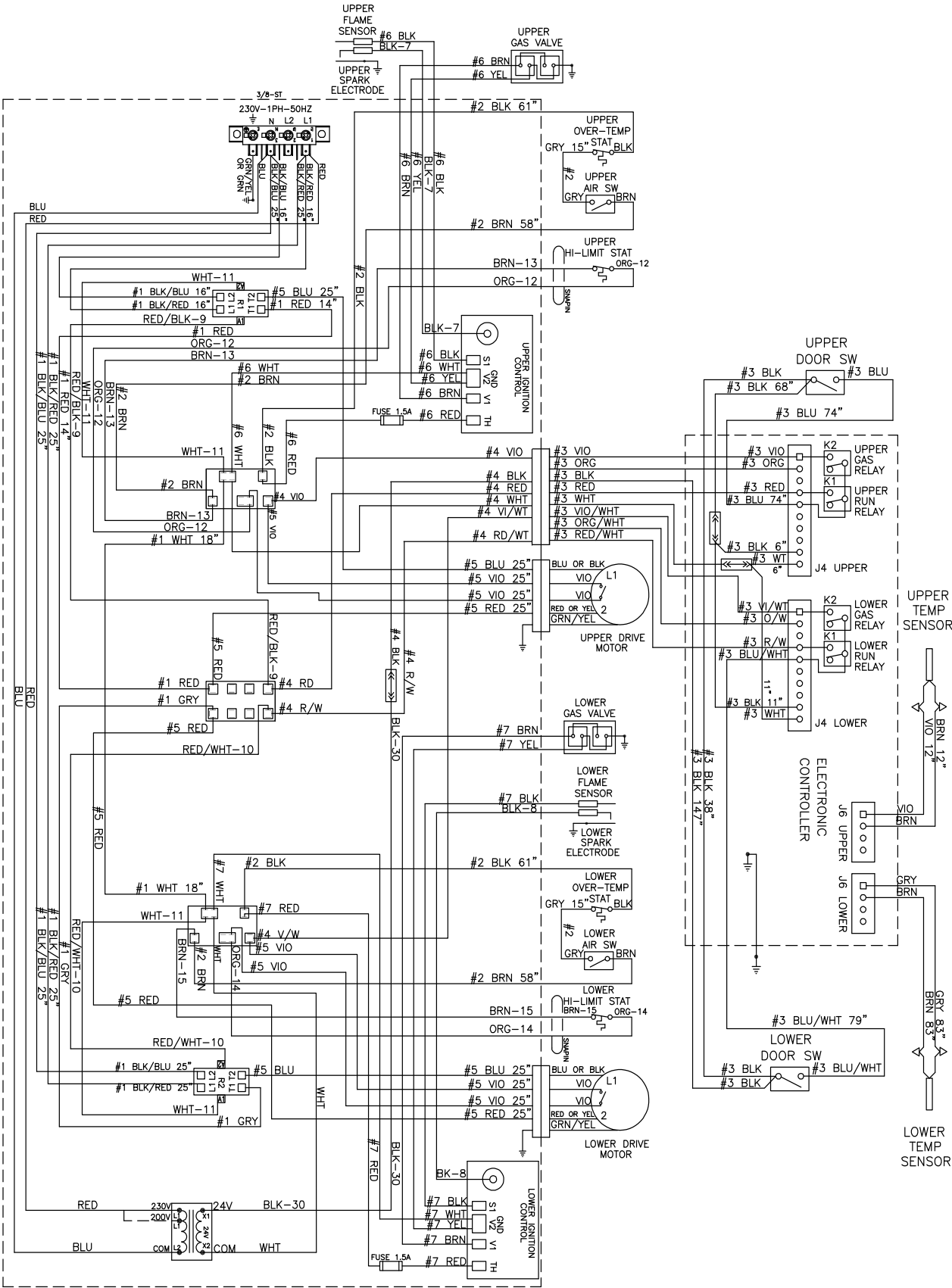
9506-825-001C WIRING DIAGRAM DN(30/50)X2N_-39_B2X-
