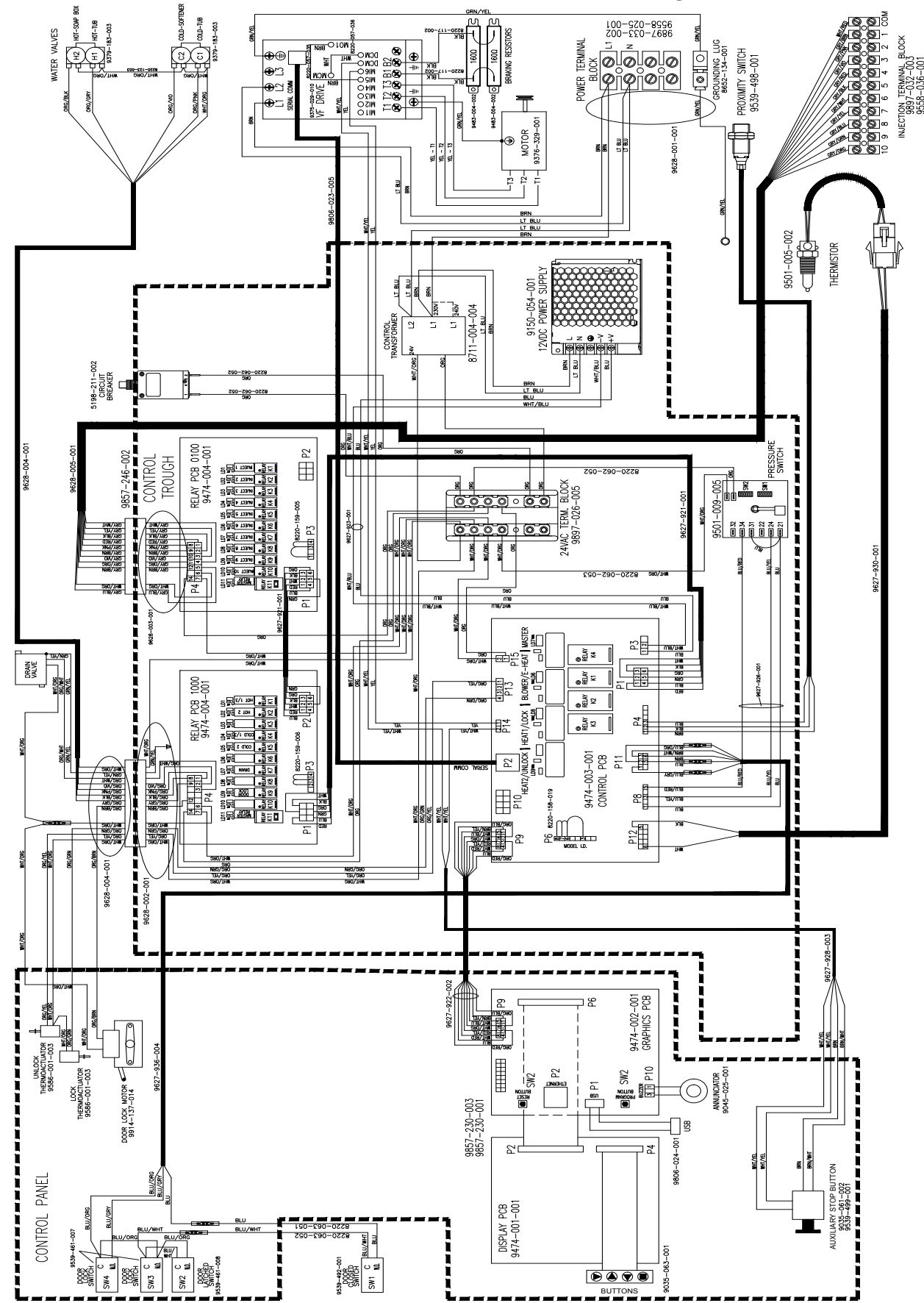
WN0750XB-39XO1 Diagram
