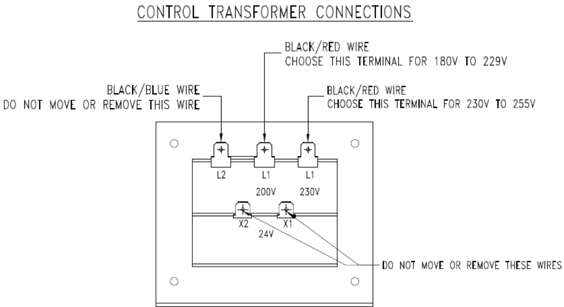
50 Hz Control Transformer Connections
