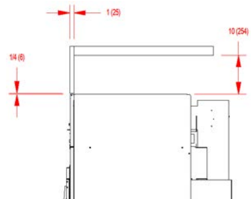
VERTICAL CLEARANCE DIMENSIONS - ALL (30/50/80/120)
