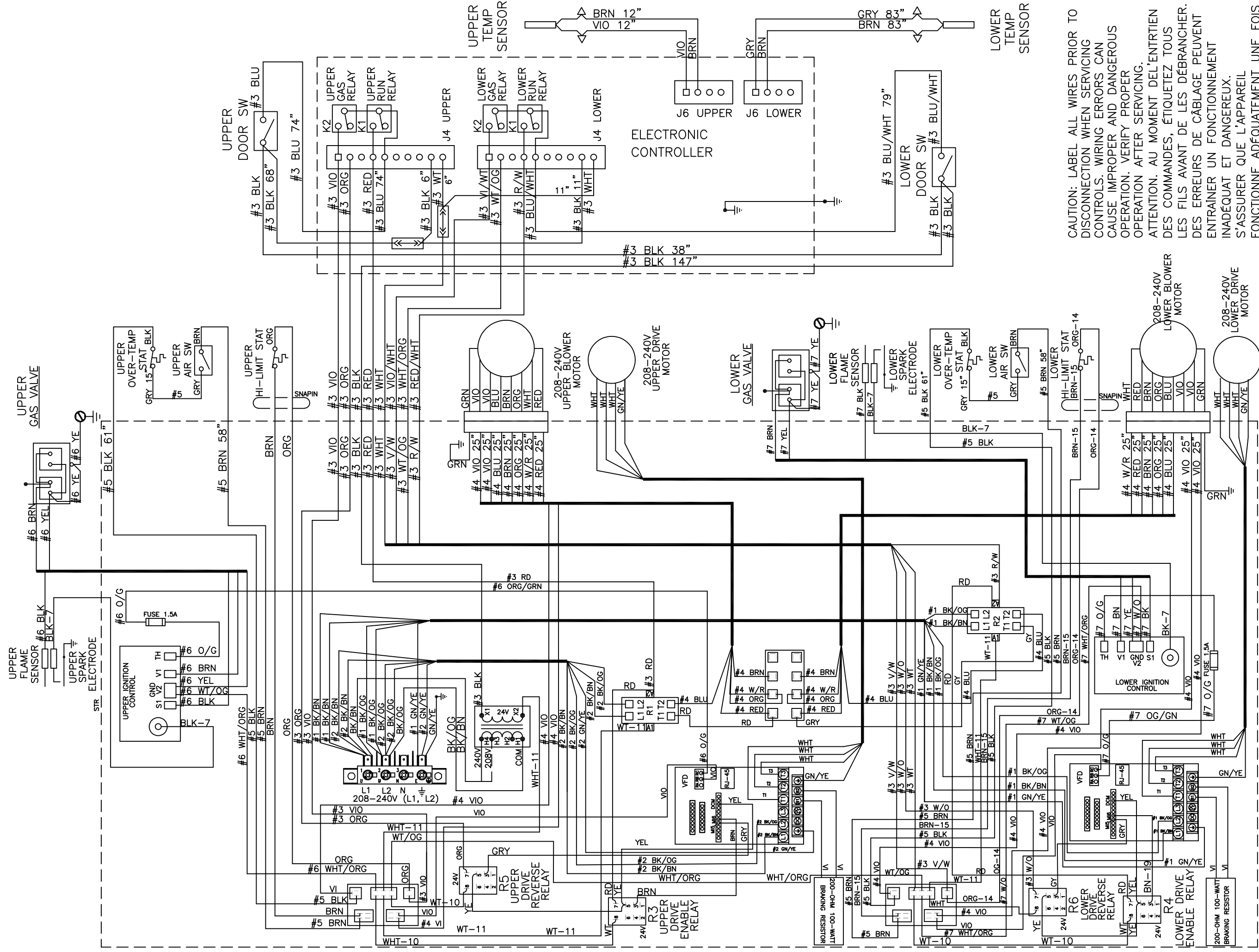
9506-981-001B WIRING DIAGRAM DN50X2N-11_B_R
