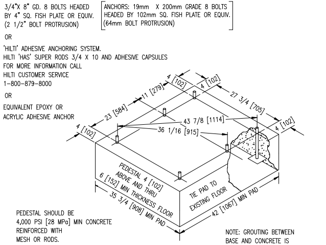
FLOOR OUTLINE Figure 1-2
