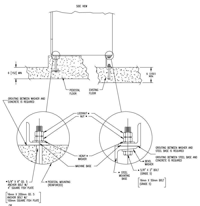
MACHINE MOUNTING DETAIL Figure 1-3
