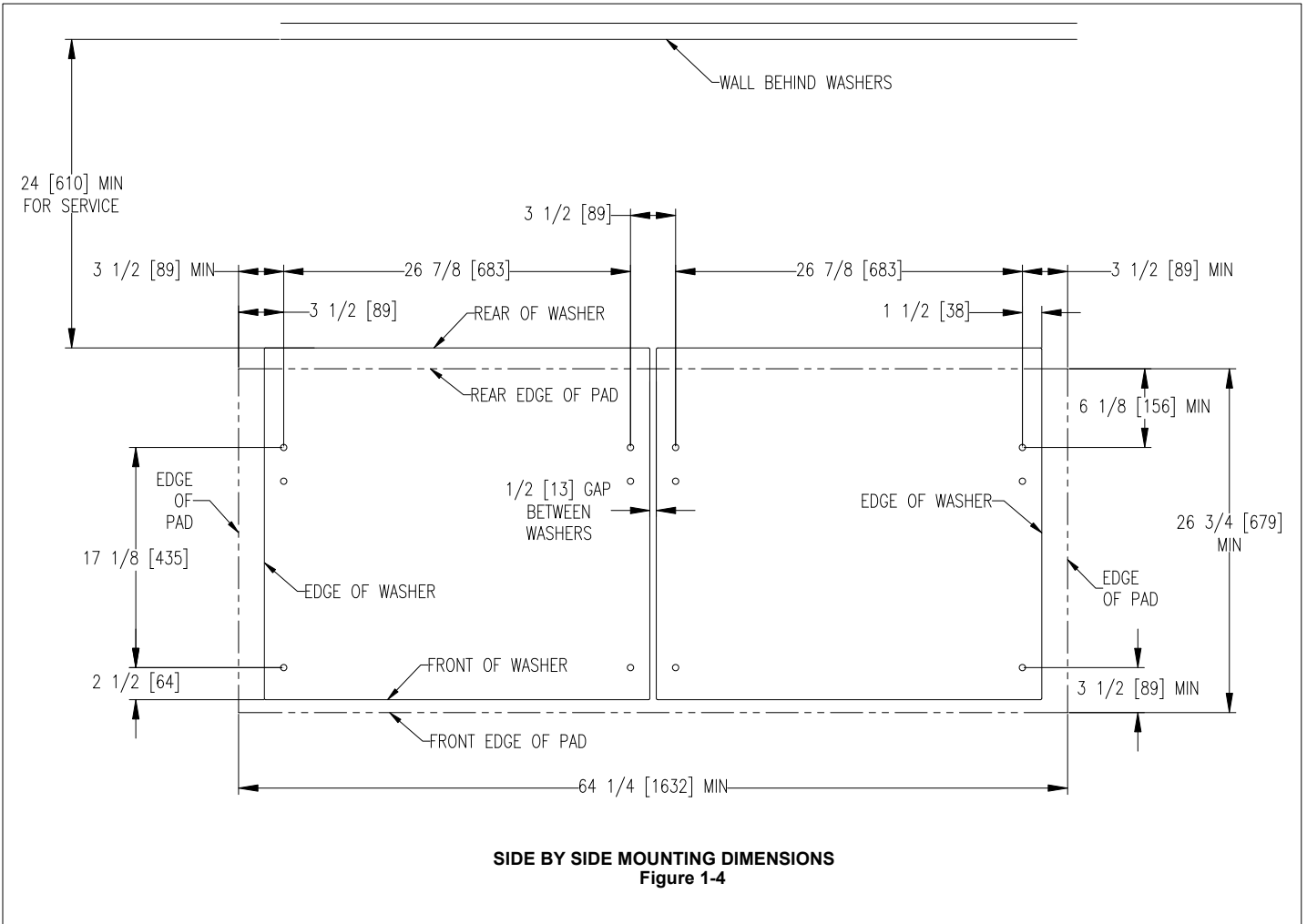
T-400 Machine Side By Side Mounting Detail
