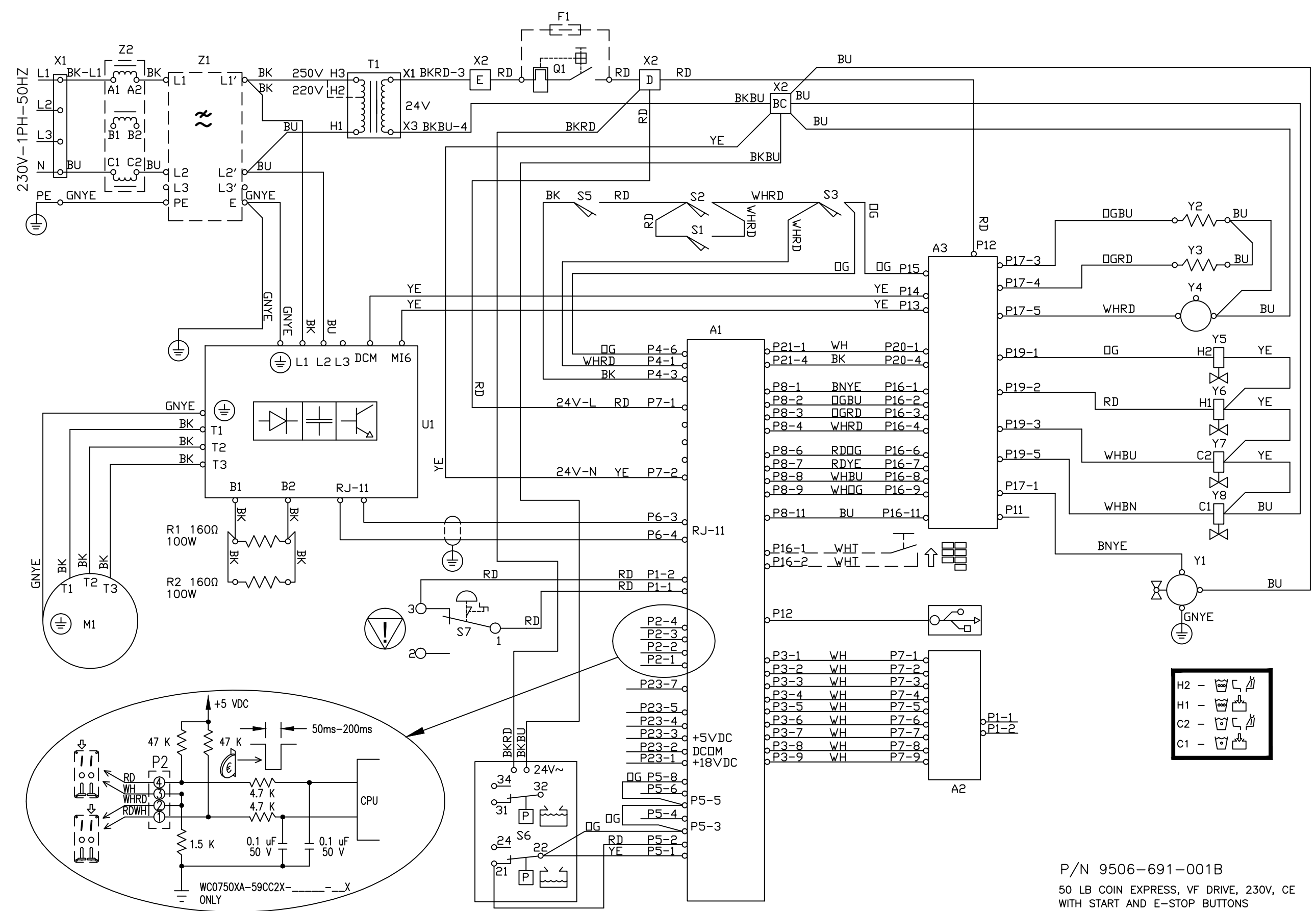
SCHMATIC 230V-1PH-50HZ
