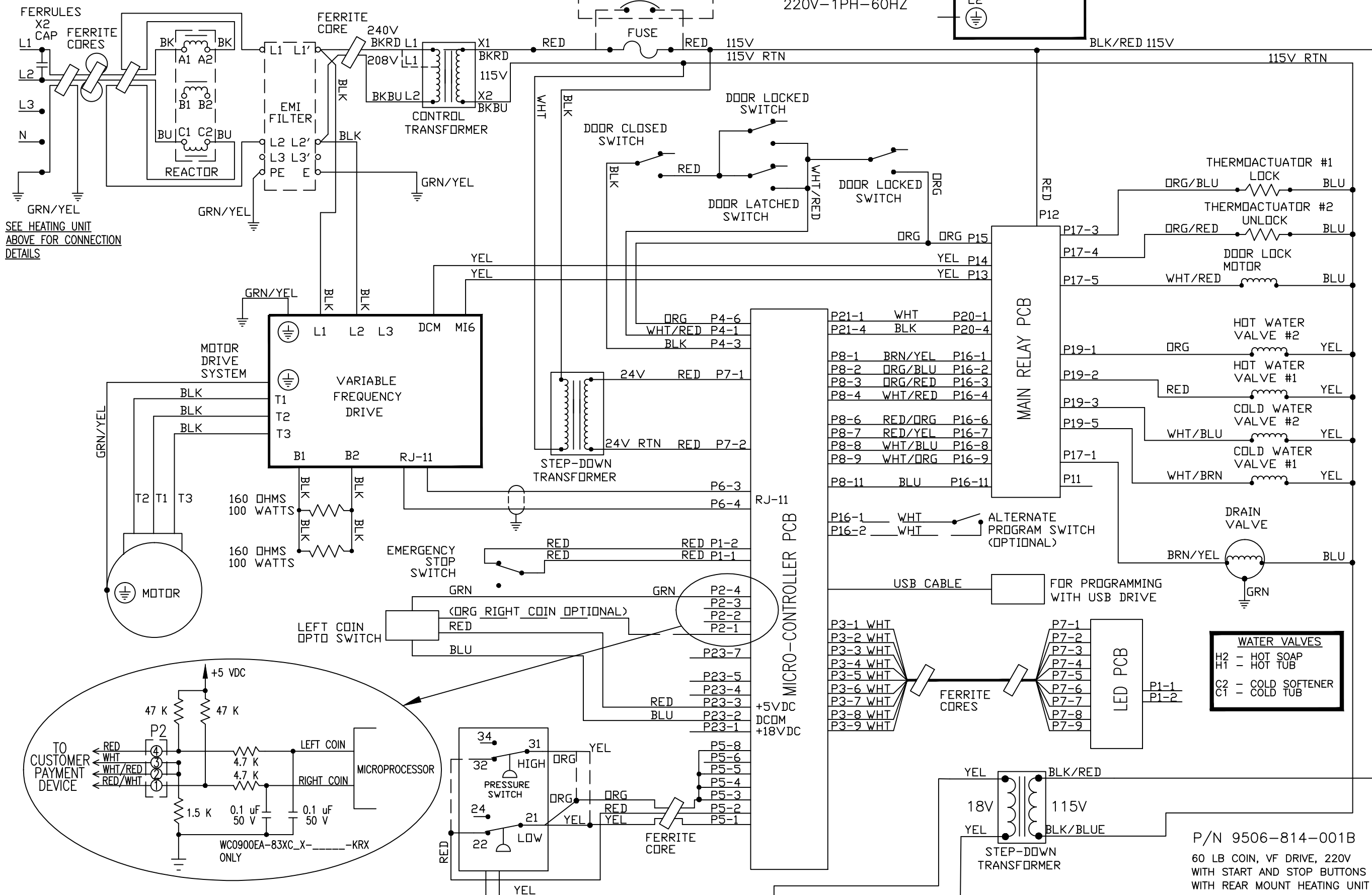
SCHEMATIC 220V-1PH-60HZ
