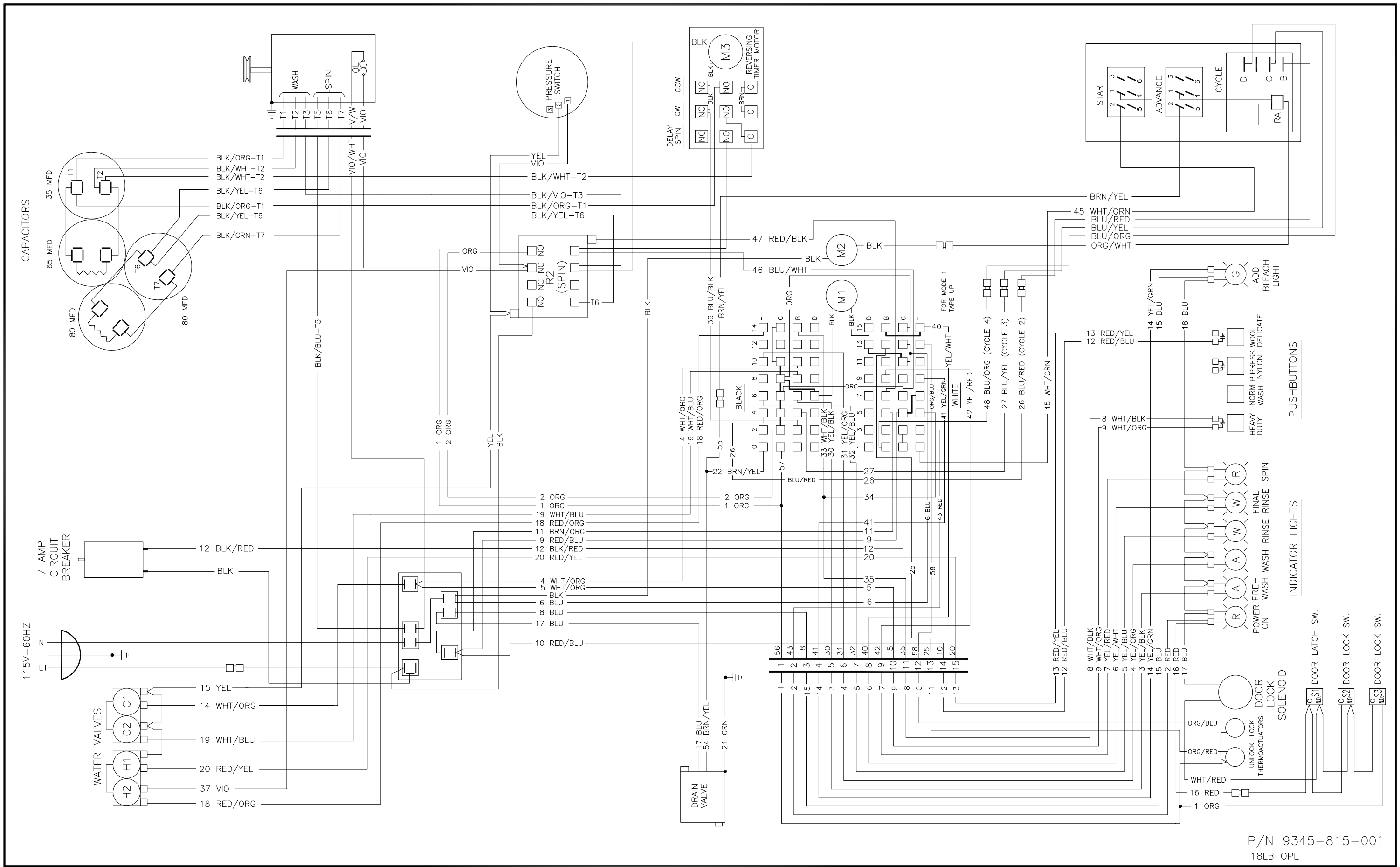
WIRING DIAGRAM 115V-1PH-60HZ
