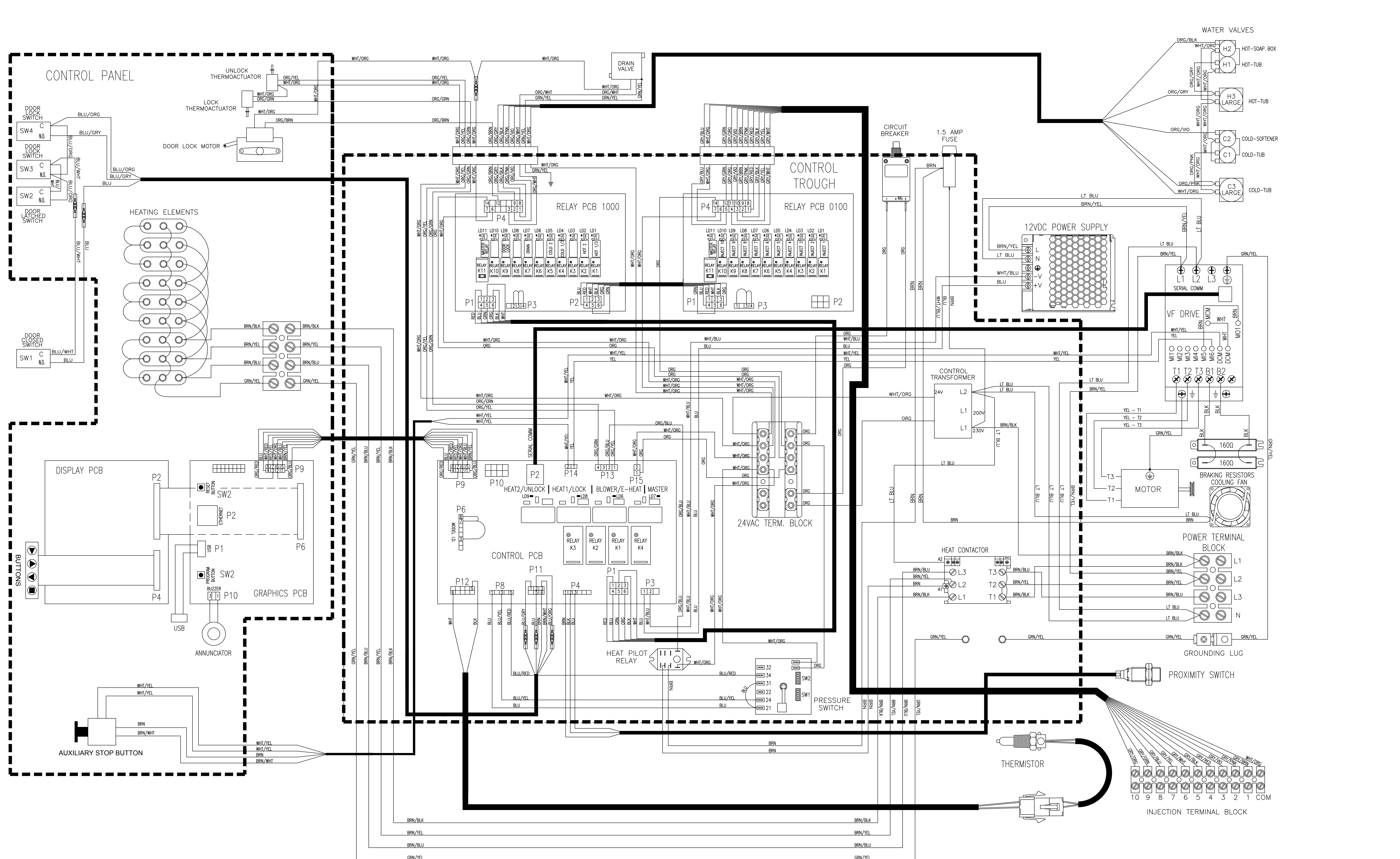
WIRING DIAGRAM 400V, 3PH, 50HZ
