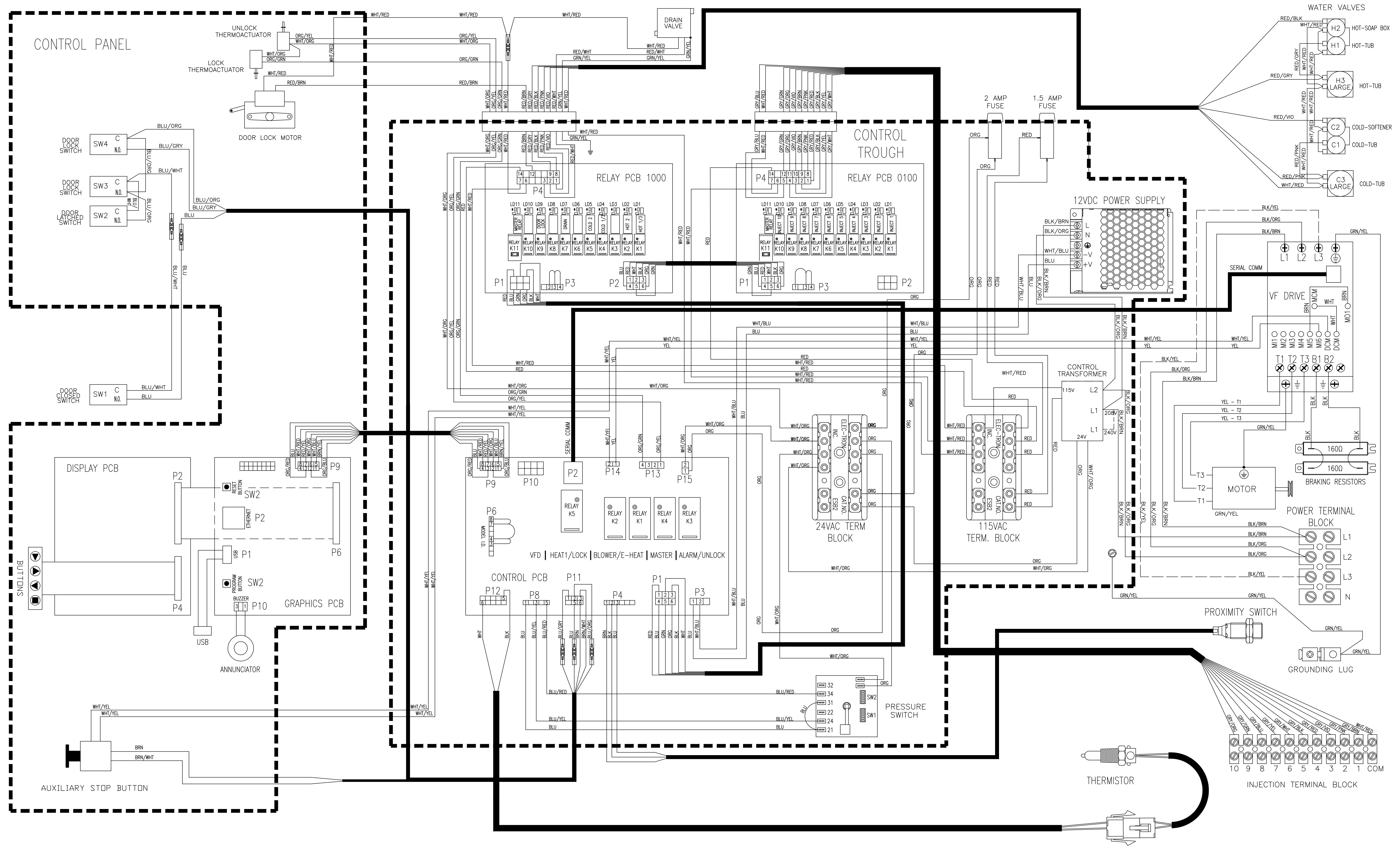
WIRING DIAGRAM 208 - 240V, 1/3PH, 60HZ
