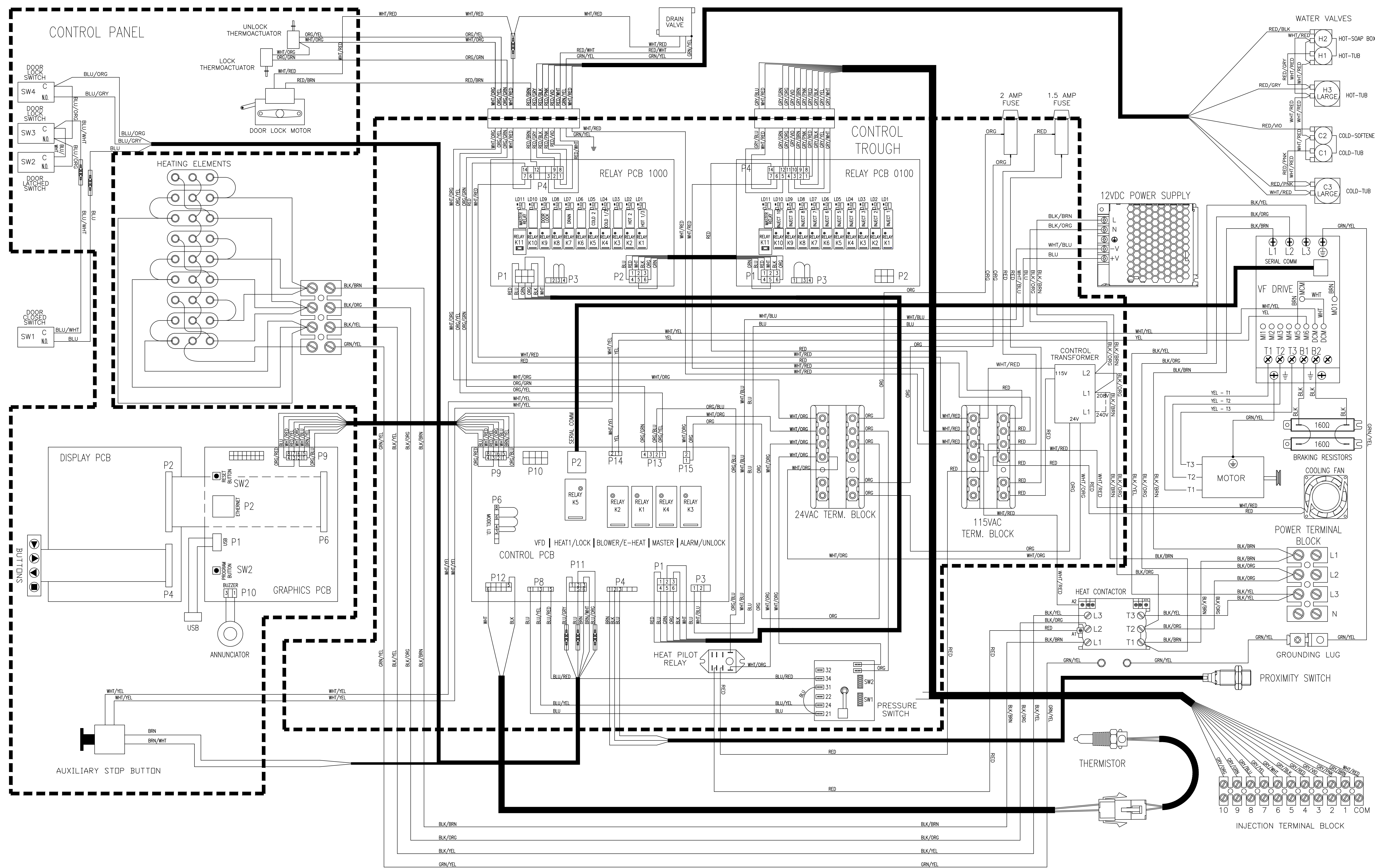
WIRING DIAGRAM 208 - 240V, 3PH, 60HZ
