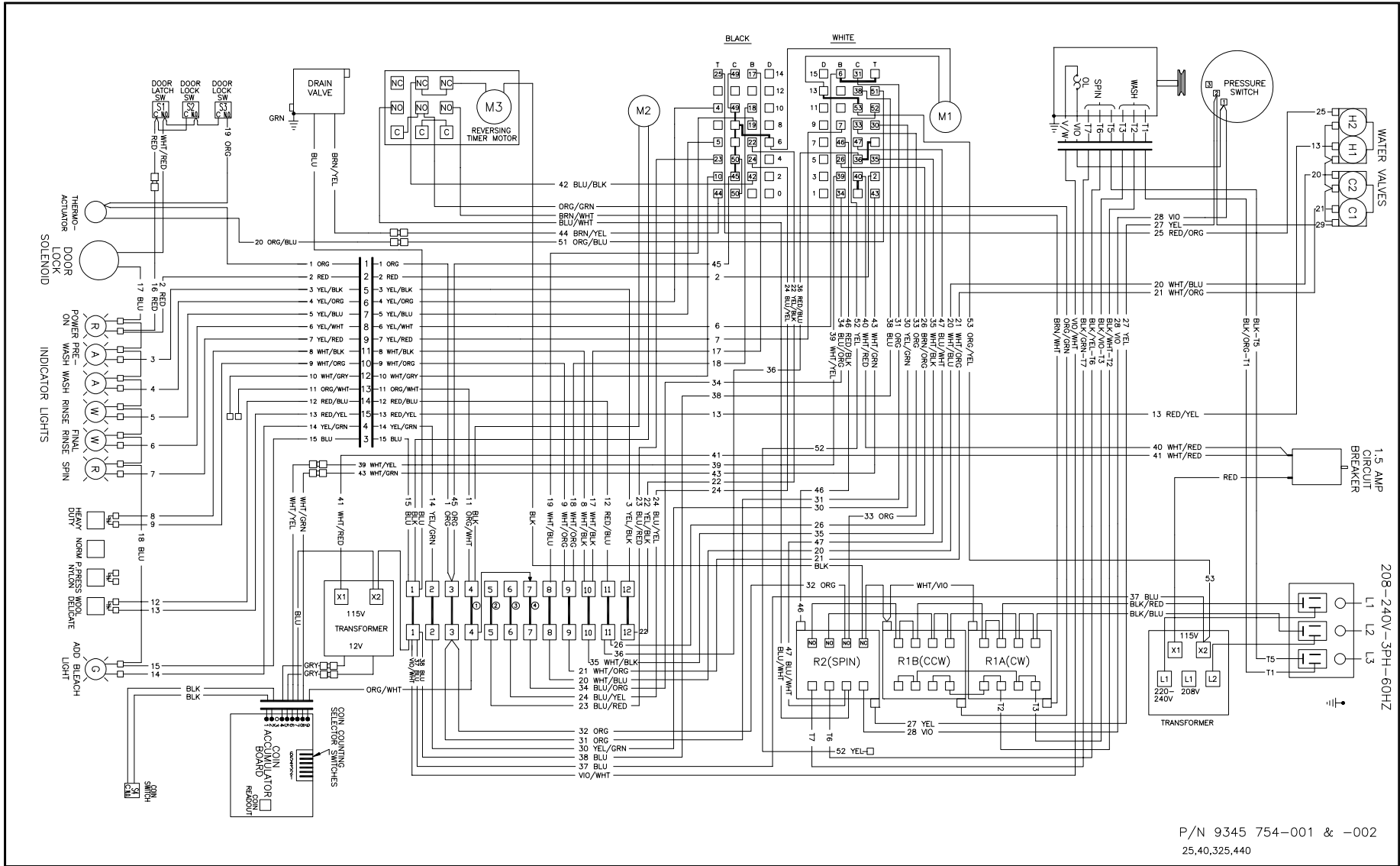
WIRING DIAGRAM 208-240V-3PH-60HZ
