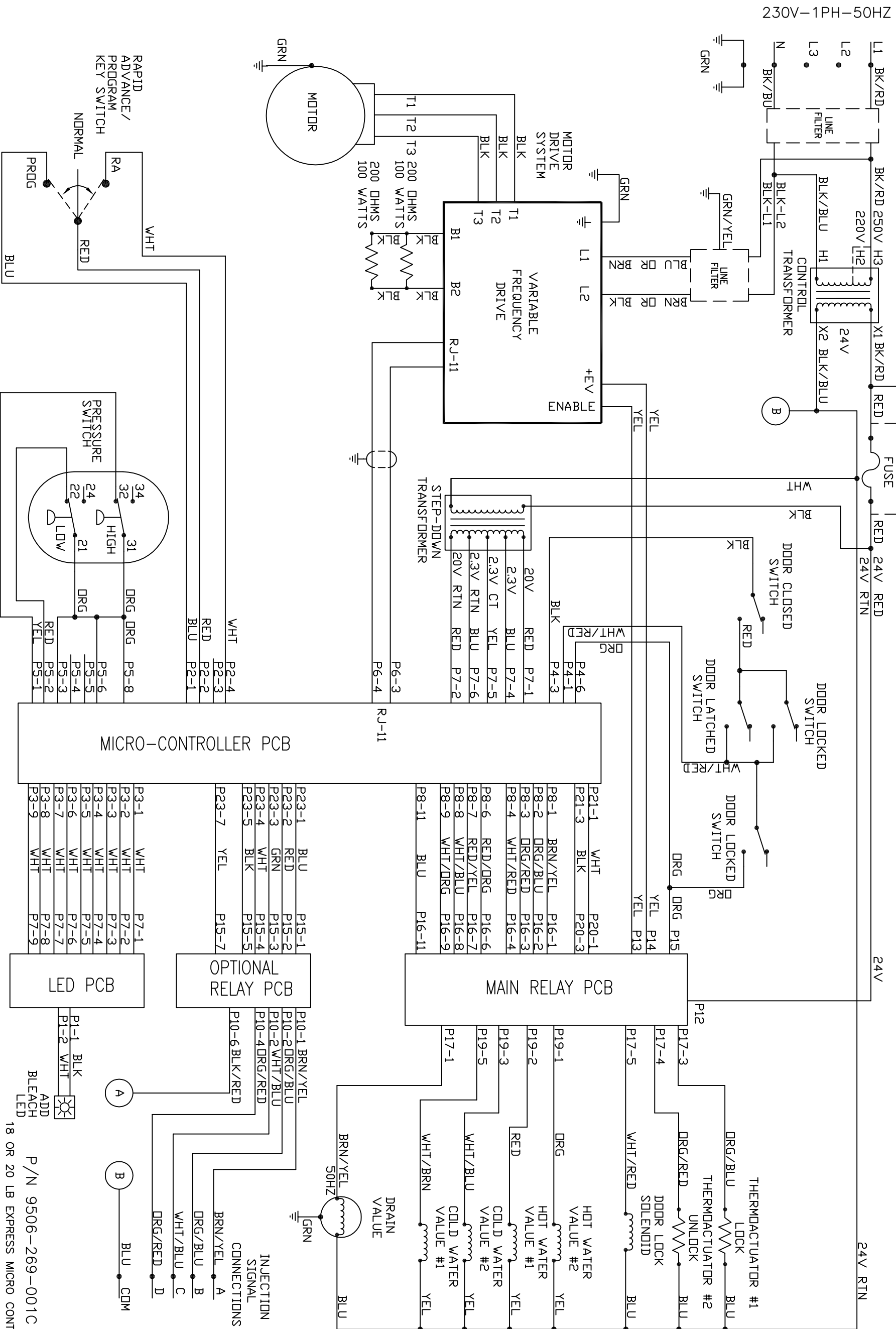
SCHEMATIC 230V-1PH-50HZ
