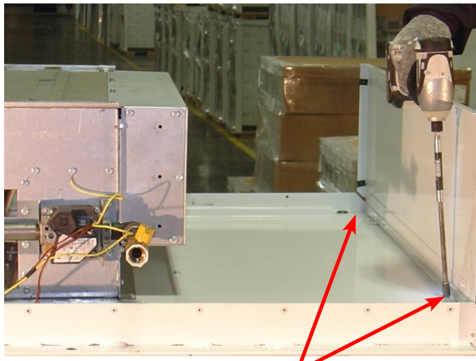
5/16 head screws
