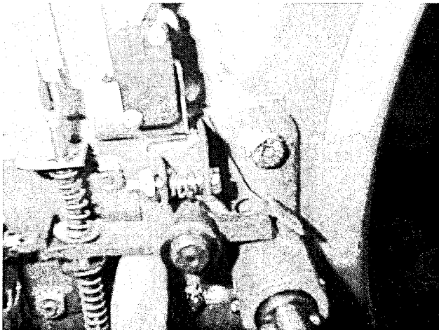
PHOTO # 7 SHOWS LOCK ARM ENGAGED
