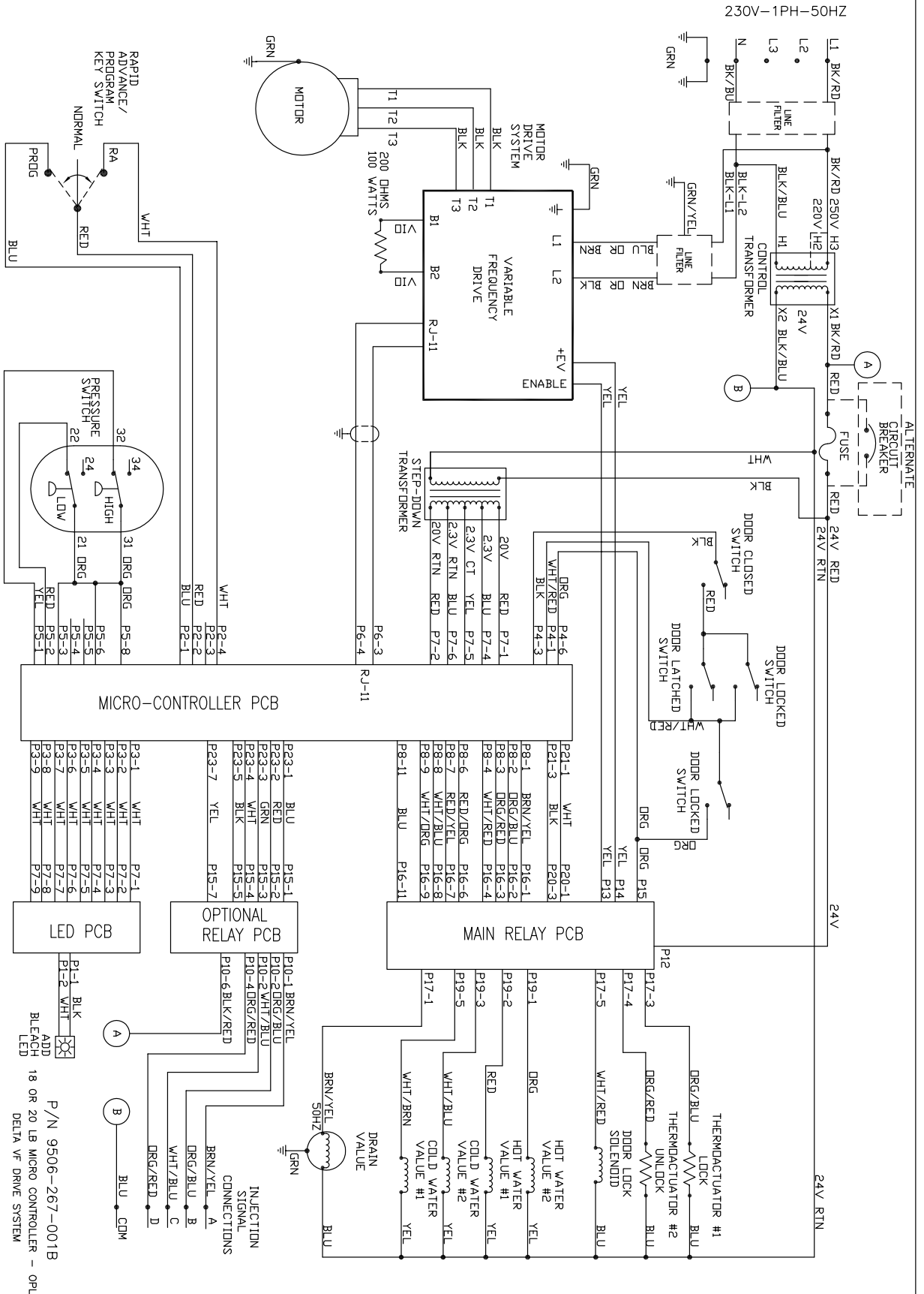
SCHEMATIC 230V-1PH-50HZ
