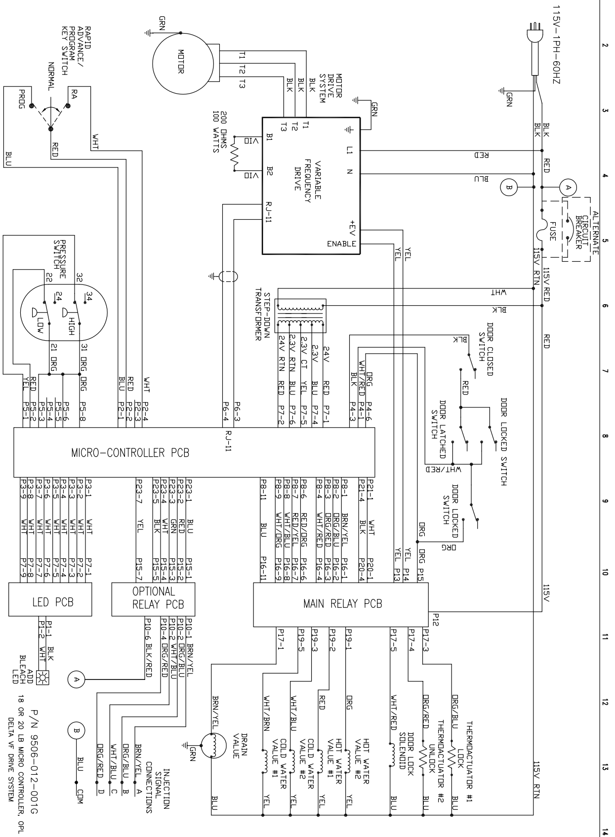
SCHEMATIC 115-1PH-60HZ
