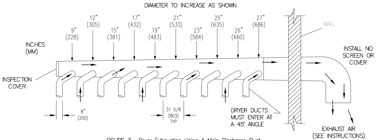
FIGURE 3— Dryer Exhausting Using A Main Discharge Duct.
