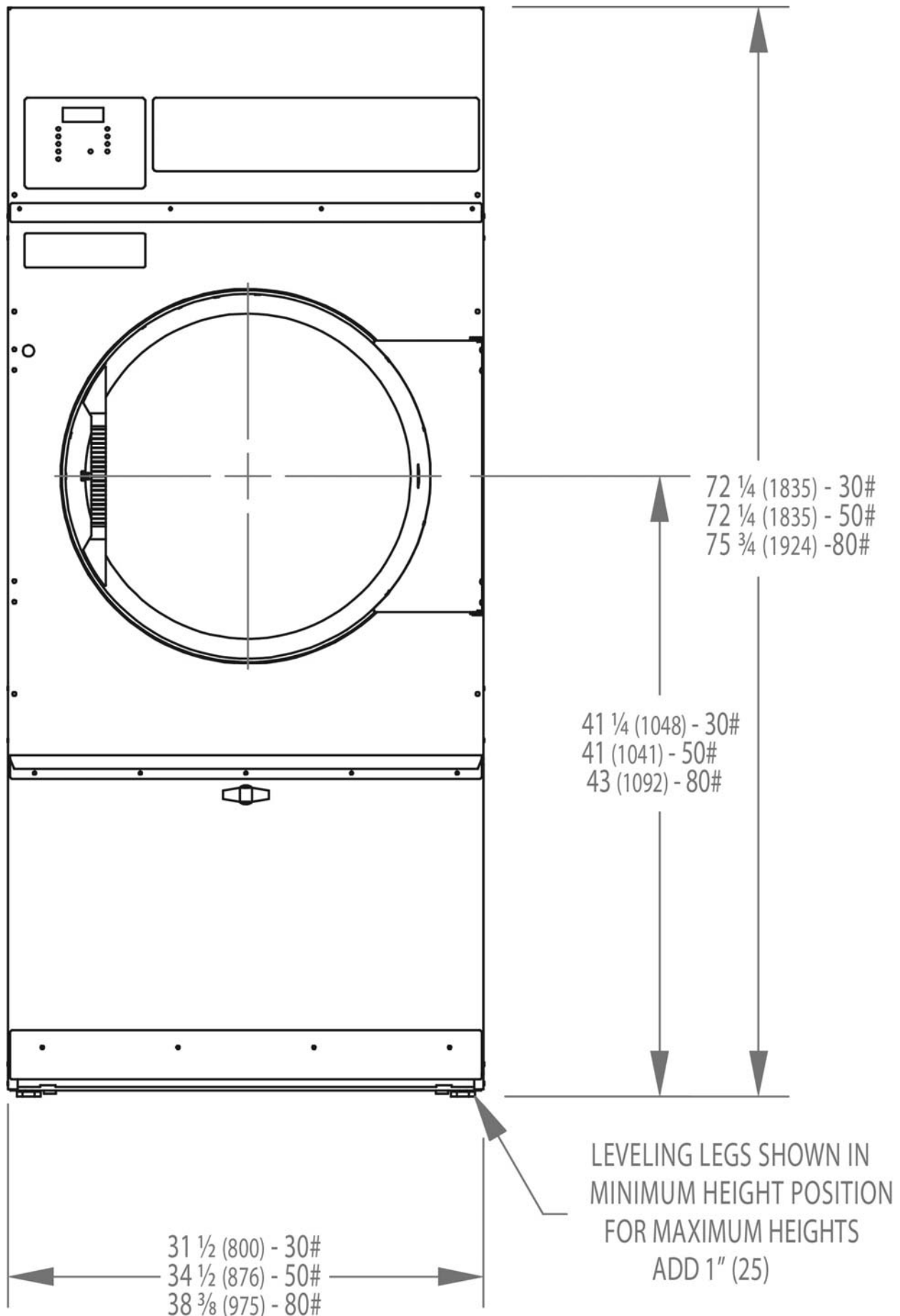
DRYER DIMENSIONS - FIGURE 1A
