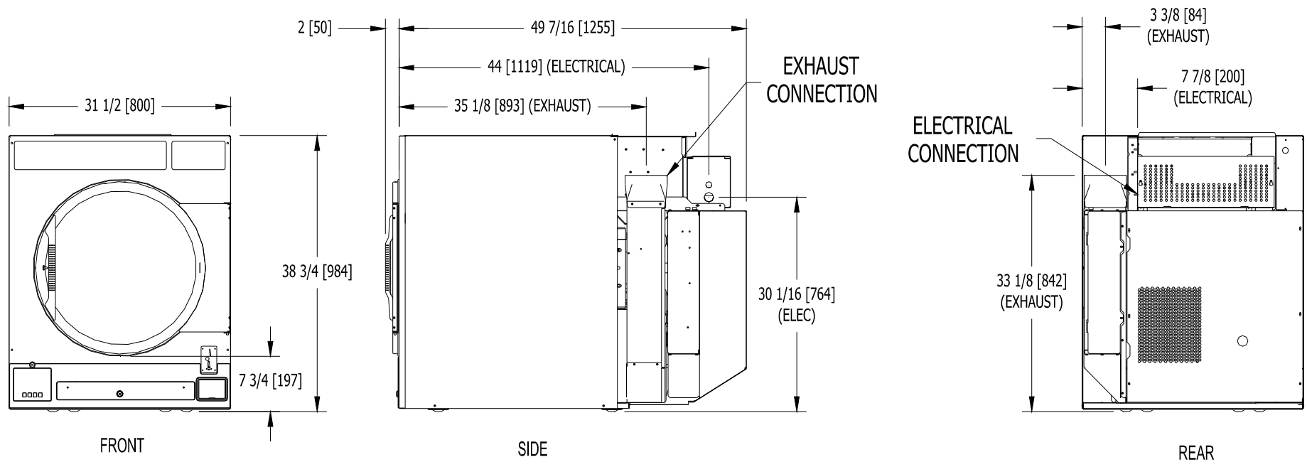
FIGURE 1 – DRYER DIMENSIONS inches [mm]
