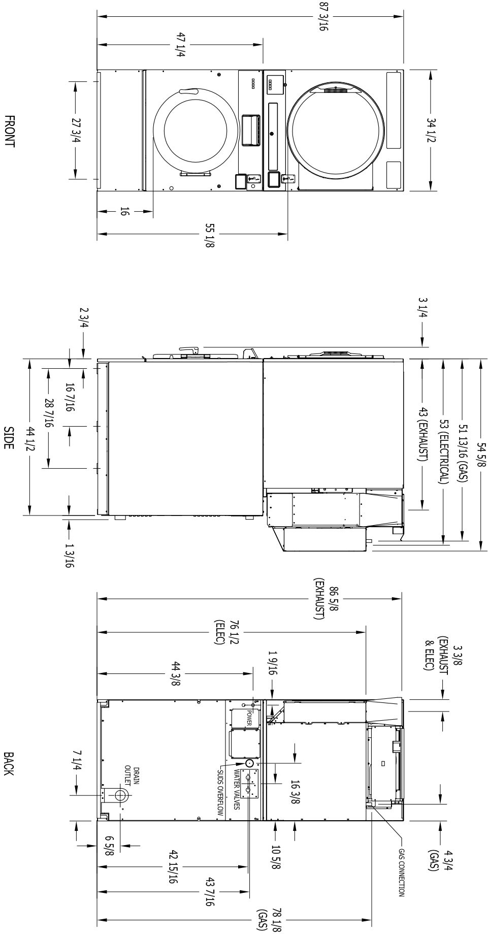
T-750 SMD COMMERCIAL STACK WASHER/DRYER MOUNTING DIMENSIONS
